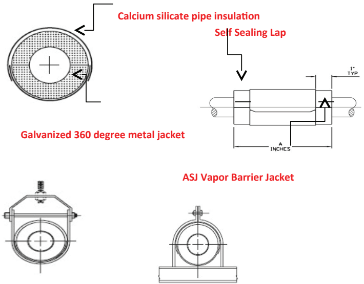
CLEVIS HANGER
