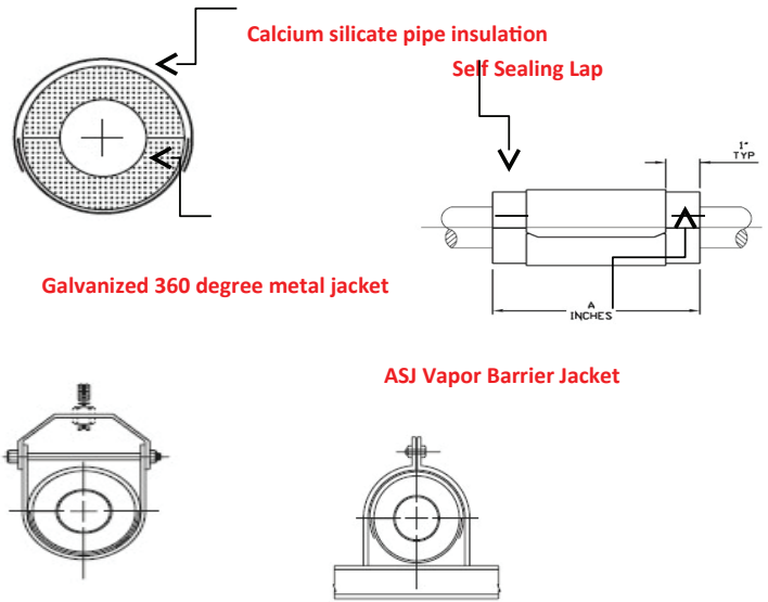
CLEVIS HANGER
